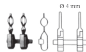
MÜLLER 45-119 Kapanma kuvveti/Closing force. 25-30 gr.
