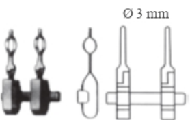
MÜLLER 45-118 Kapanma kuvveti/Closing force. 25-30 gr.
